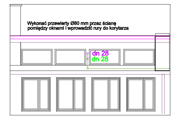
WIDOK "A"
